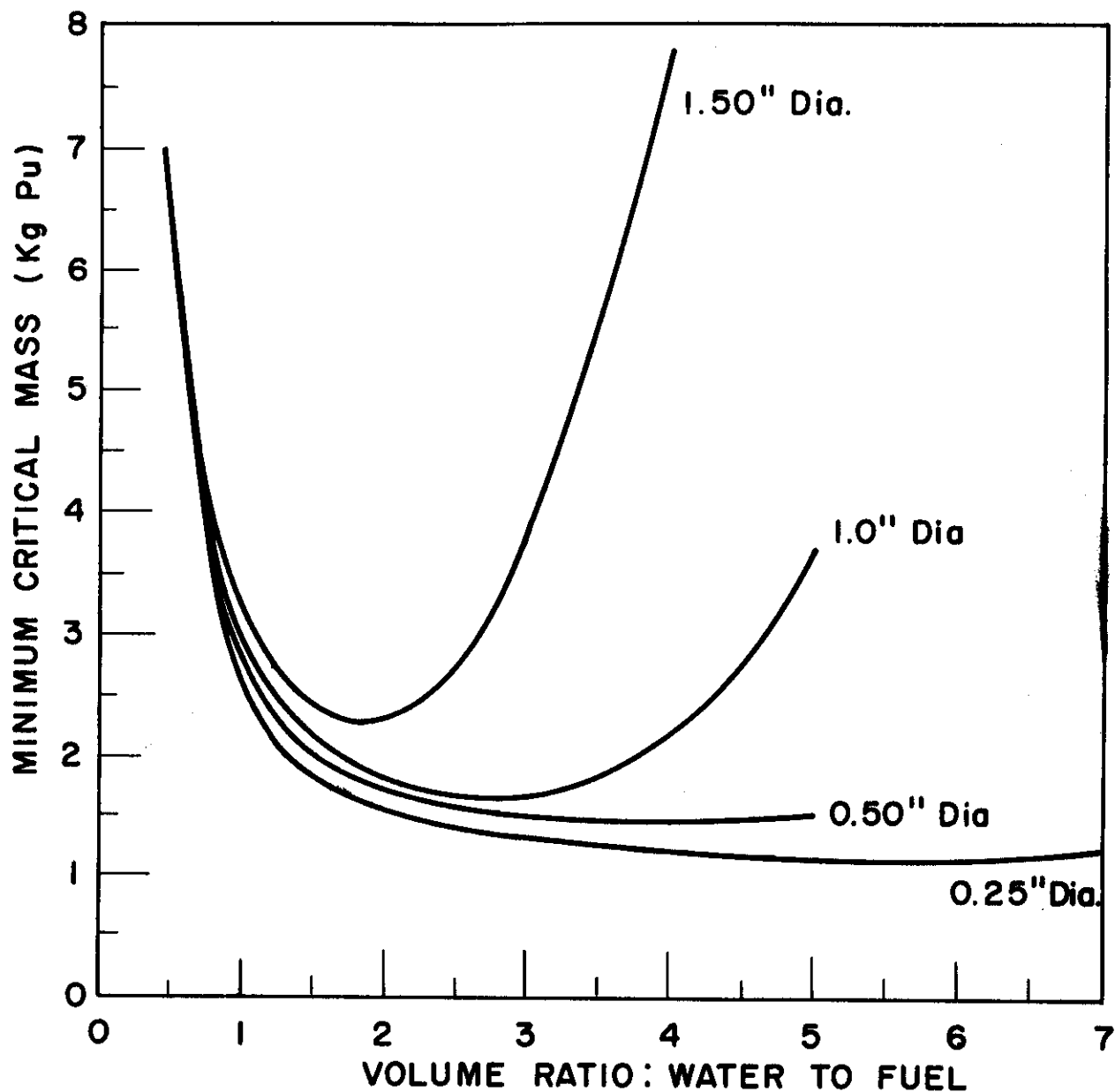
FIGURE 6 MINIMUM CRITICAL MASS vs VOLUME RATIO WATER TO FUEL (5% Pu)
