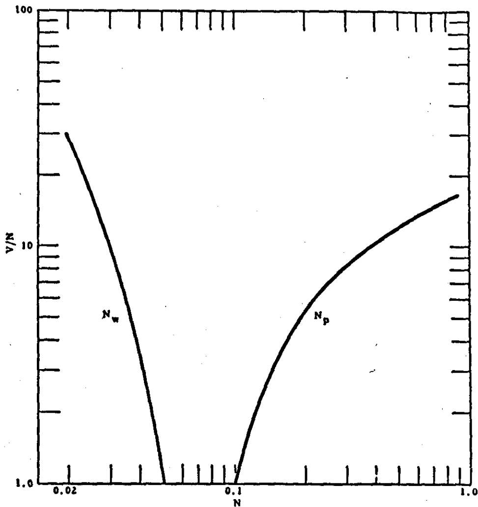
FIGURE 1 Value Function for H_c-204 ( N_0 = 0.068 )
