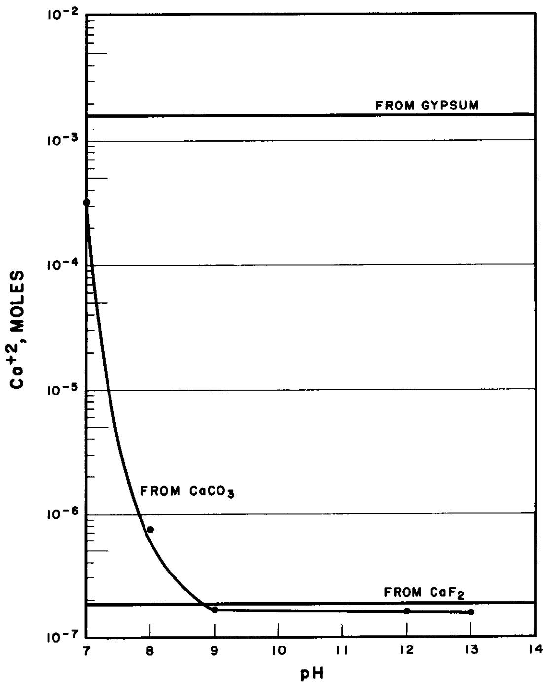
FIGURE 14 Relative Amounts of Ca 2+ from Several Compounds in Equilibrium With Indicated 0.03 M SO 4 -2 , CO 3 -2 and F - Solutions at Various H + Concentrations
