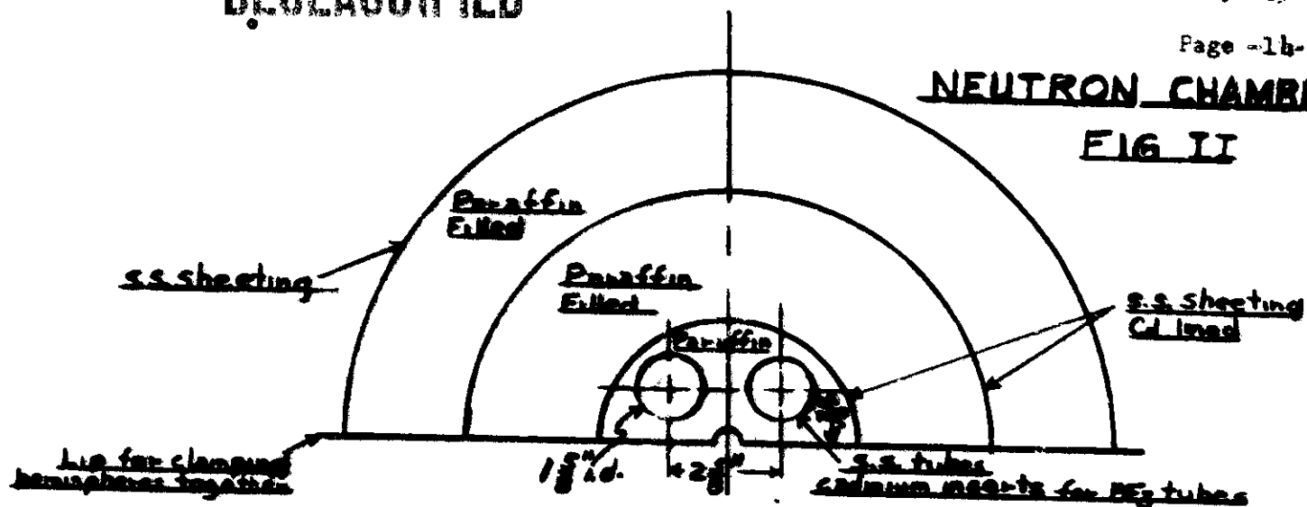
TOP VIEW ONE OF TWO IDENTICAL HEMISPHERES
