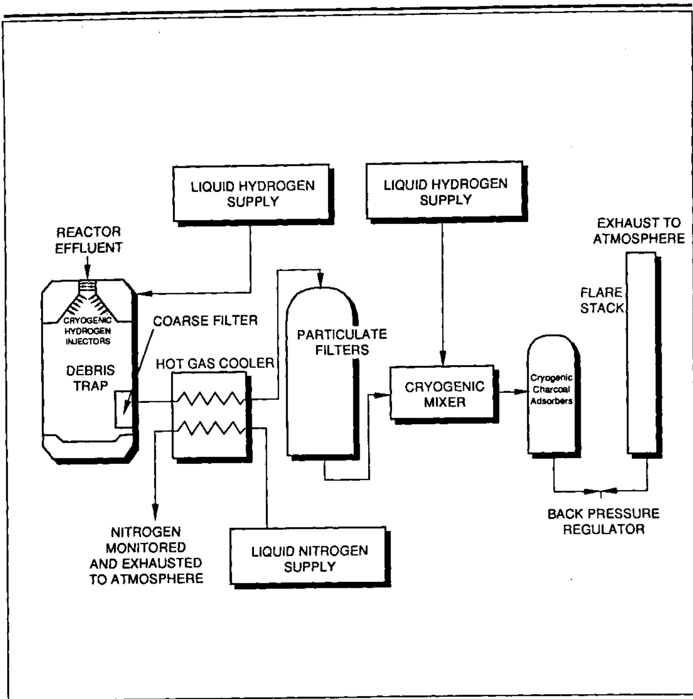
Effluent Treatment System: Conceptual Design
