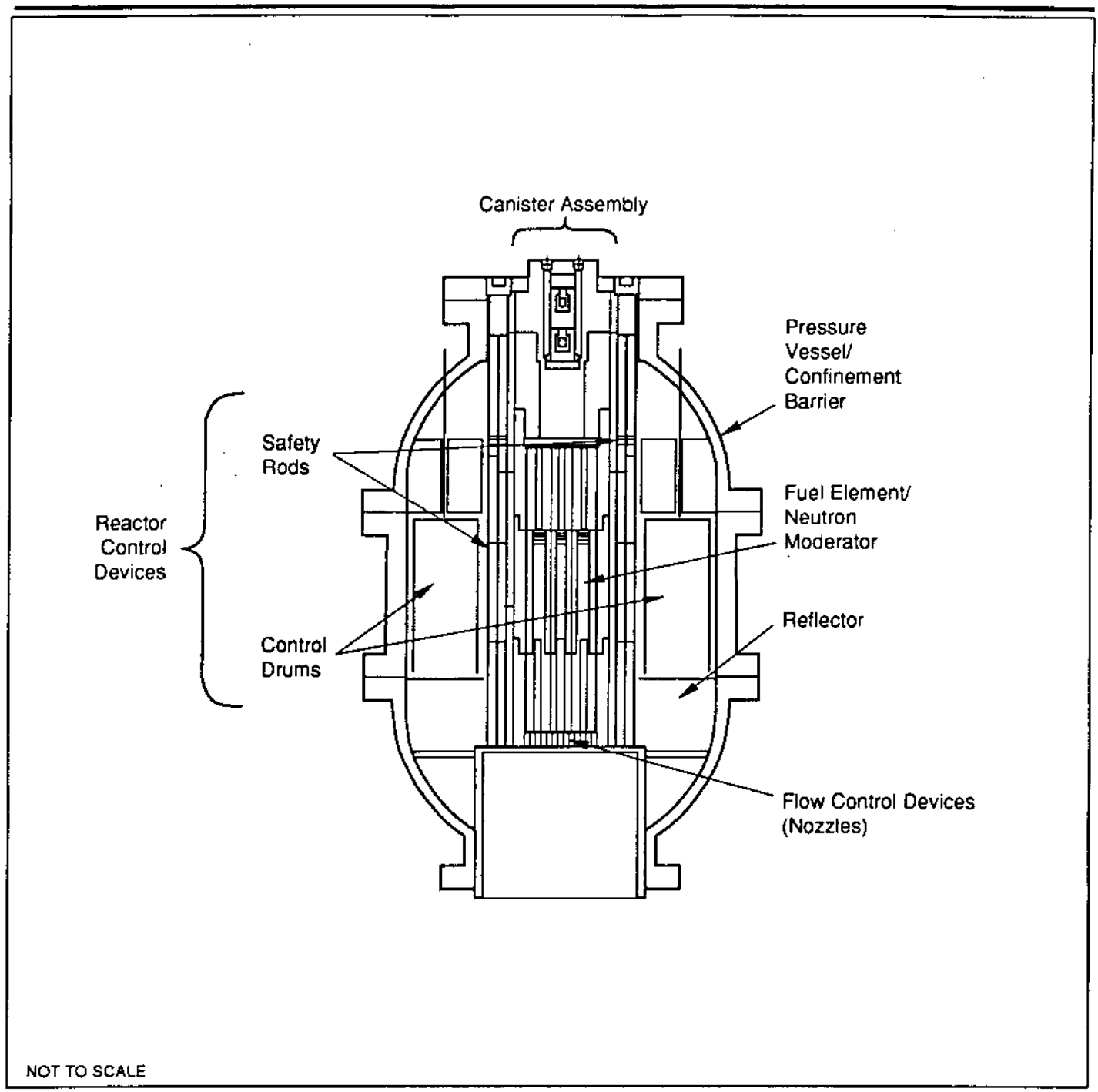
PIPET Reactor Axial Cross-Section
