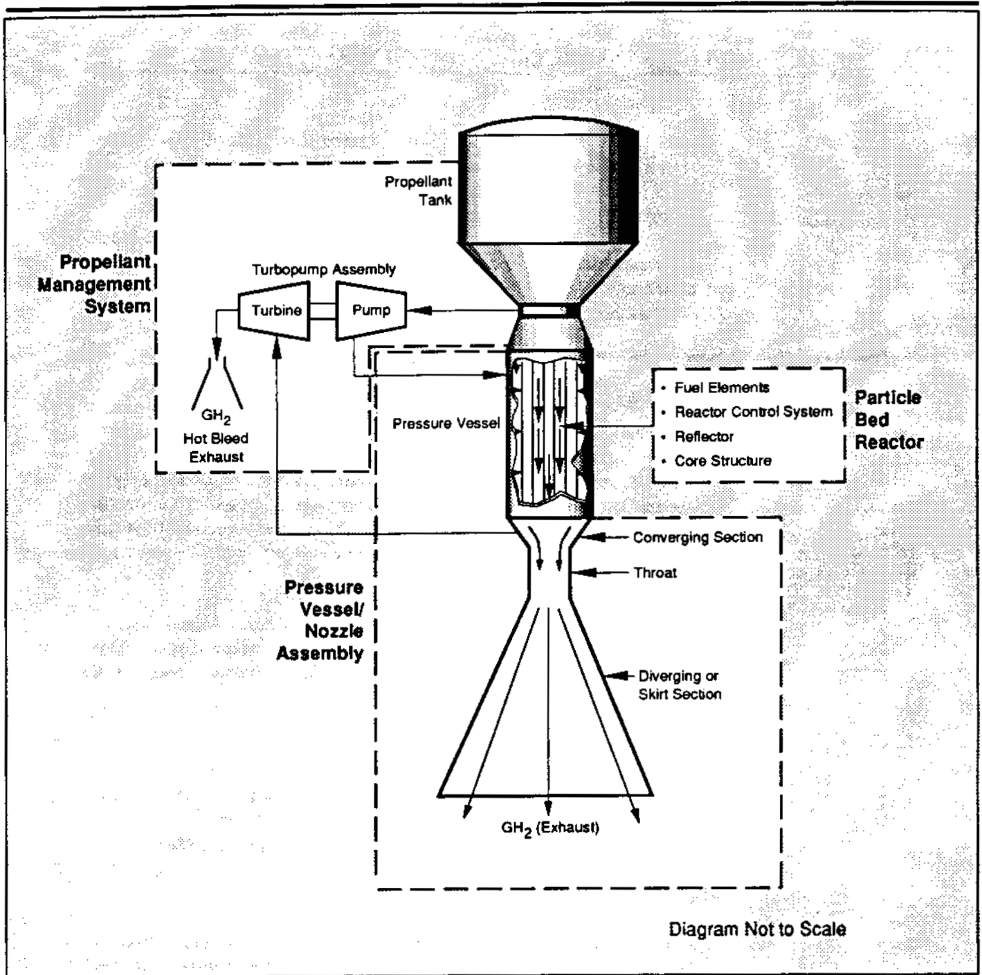
Conceptual PBR Propulsion System
