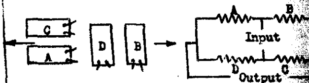
Figure B. Extremely stable - twice output of single gage.
