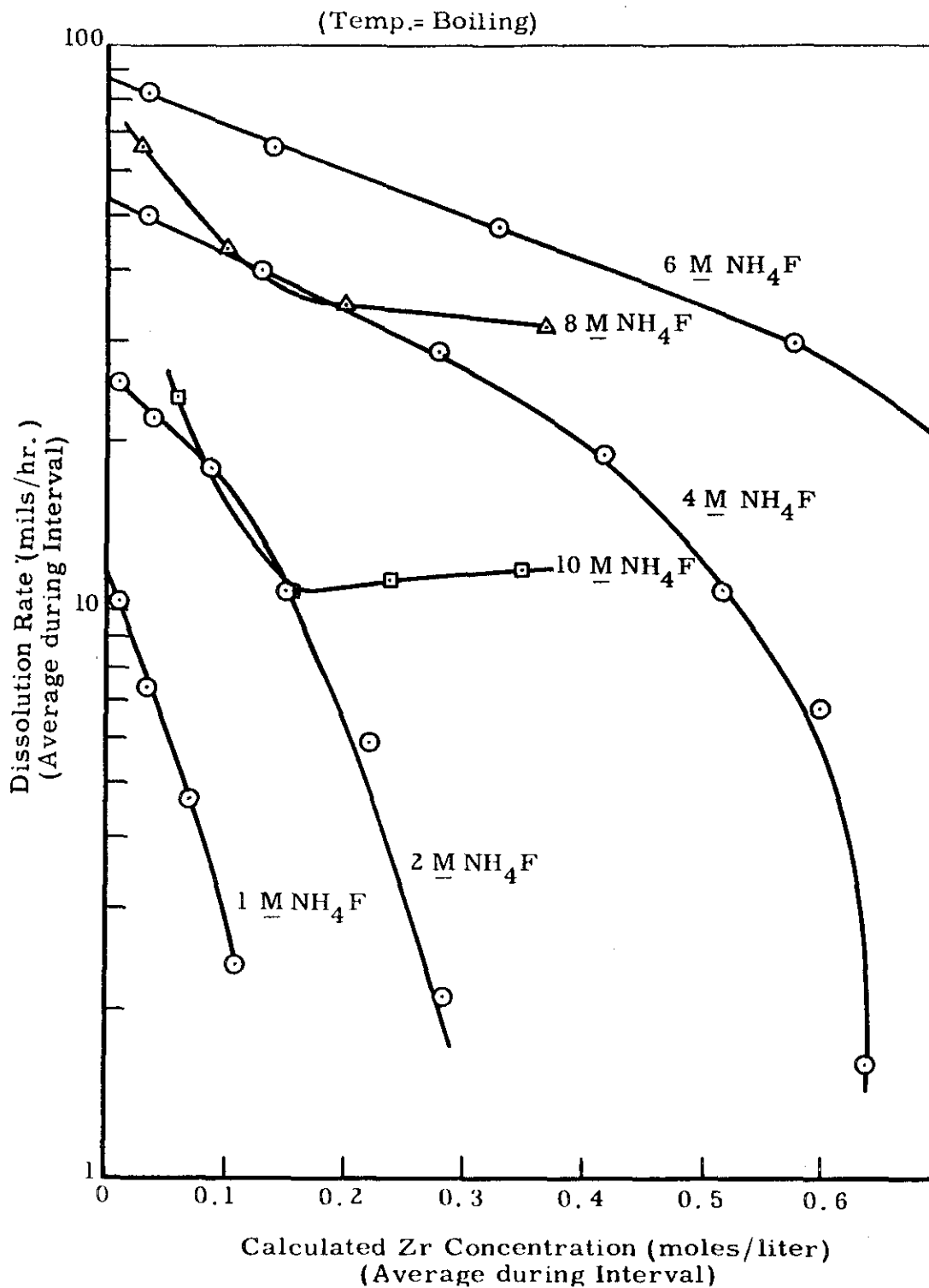
FIGURE 2 RATE OF DISSOLUTION OF ZIRCALLOY-2 IN AMMONIUM FLUORIDE SOLUTIONS
