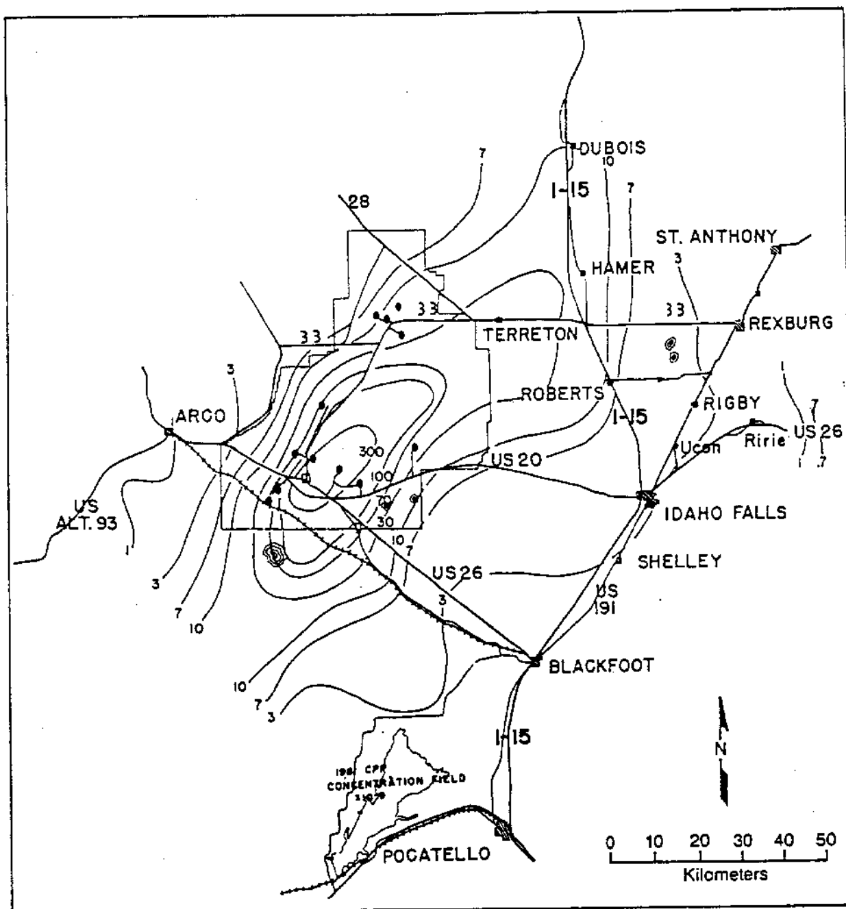
Figure B-13. 1981 average of mesoscale dispersion isopleths of air concentrations at ground level, normalized to unit release rate (DOE, 1982).
