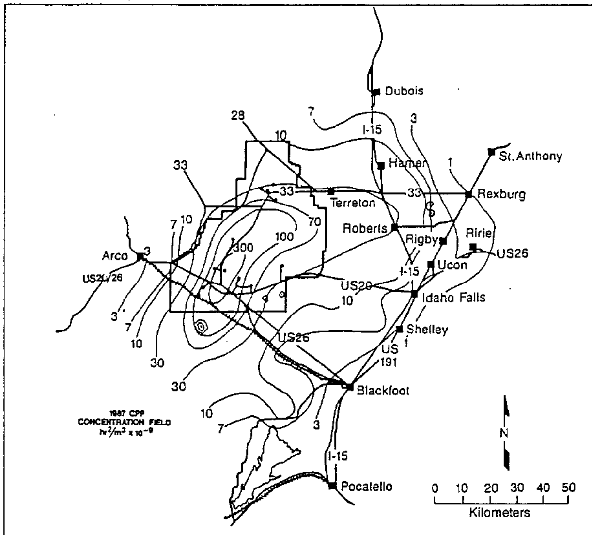
Figure B-7. 1987 average of mesoscale dispersion isopleths of air concentrations at ground level, normalized to unit release rate (Chew and Mitchell, 1988).
