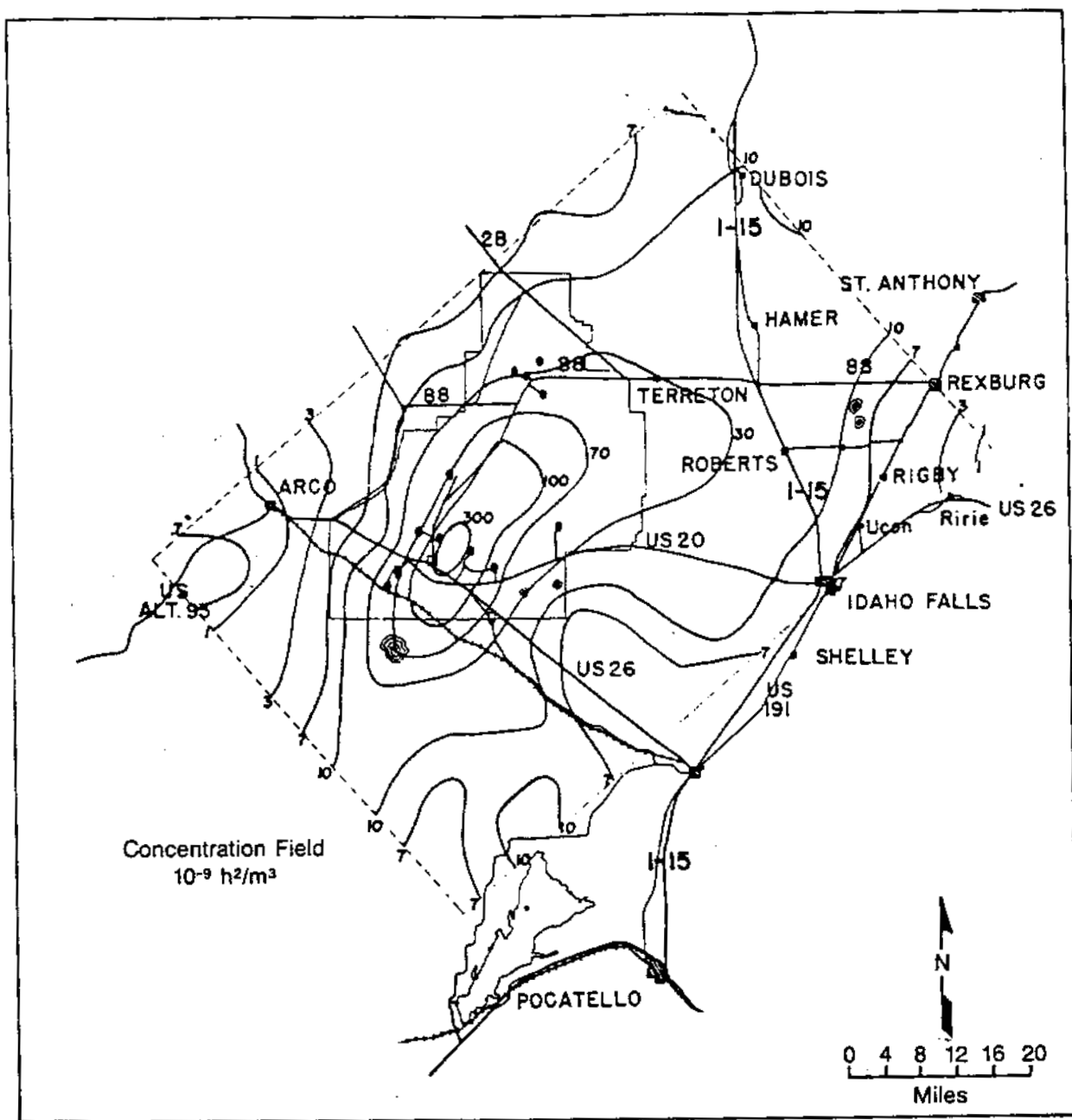
Figure B-18. 1975 average of mesoscale dispersion isopleths of air concentrations at ground level, normalized to unit release rate (ERDA, 1976).
