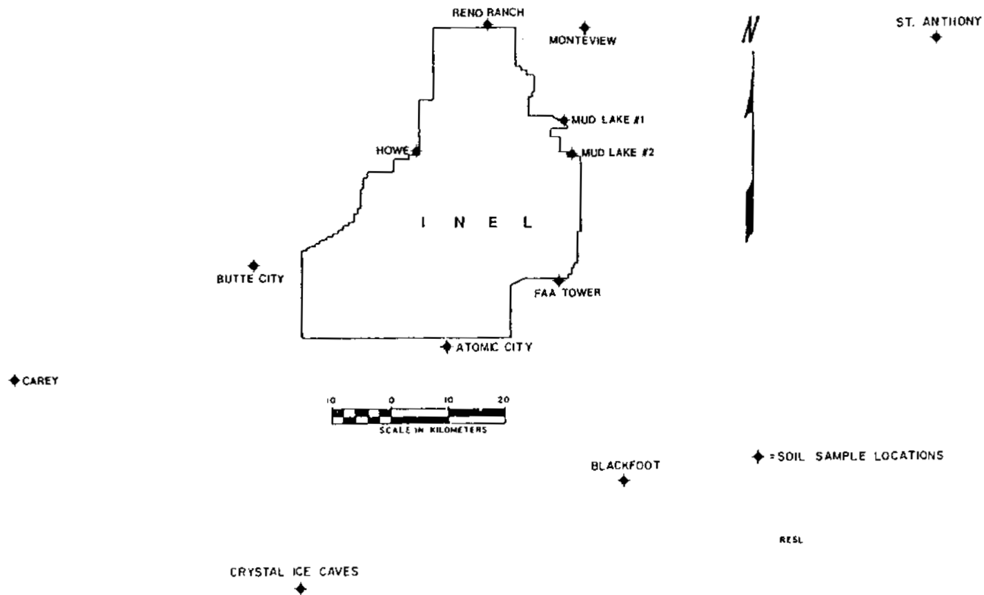
Figure E-5. Soil sampling locations for the INEL vicinity.
