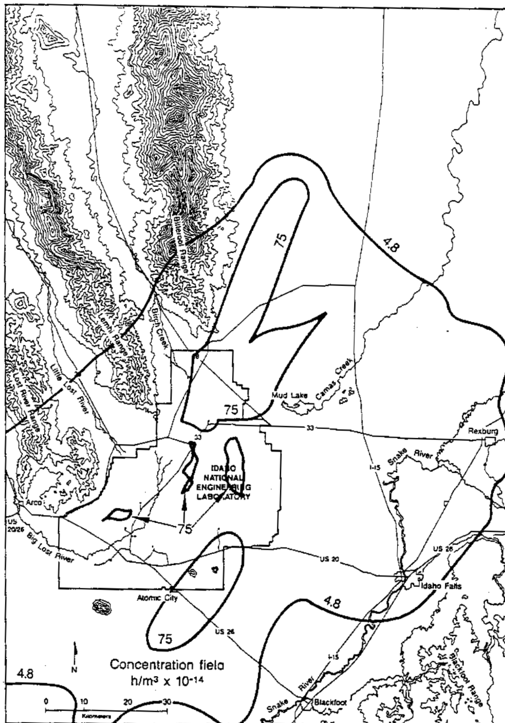
Figure B-32. Dispersion coefficient contours for IET #4(B) of 5/24-6/26/56.
