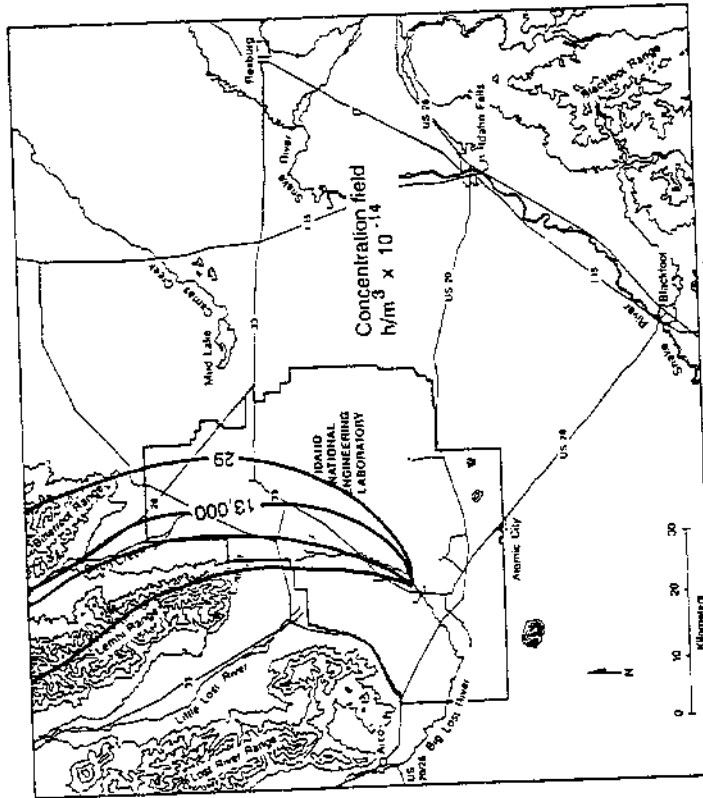
Figure B-29. Dispersion coefficient contours for Fuel Element Burn Test, B of 3/20/57.
