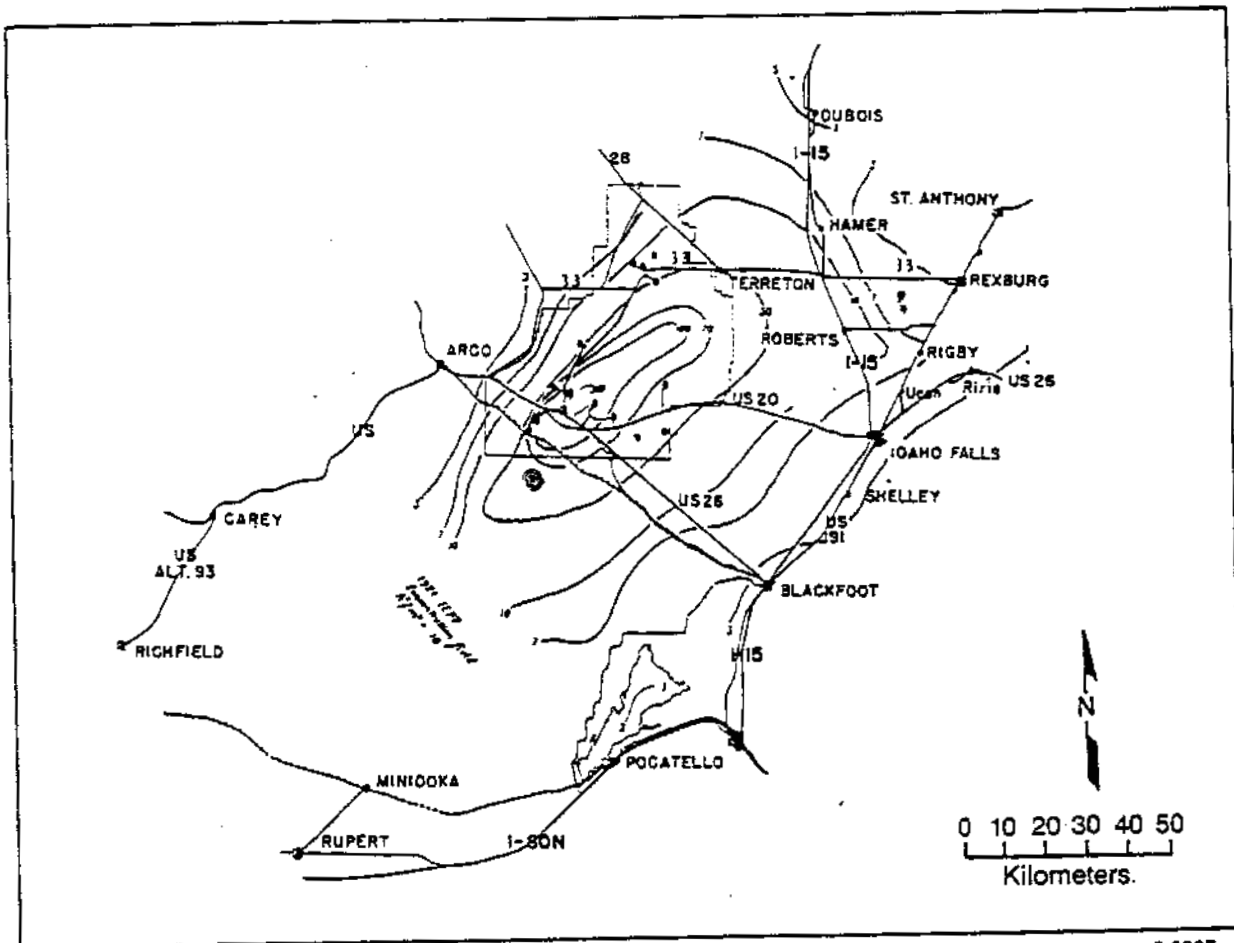
Figure B-10. 1984 average of mesoscale dispersion isopleths of air concentrations at ground level, normalized to unit release rate (Hoff et al., 1985).
