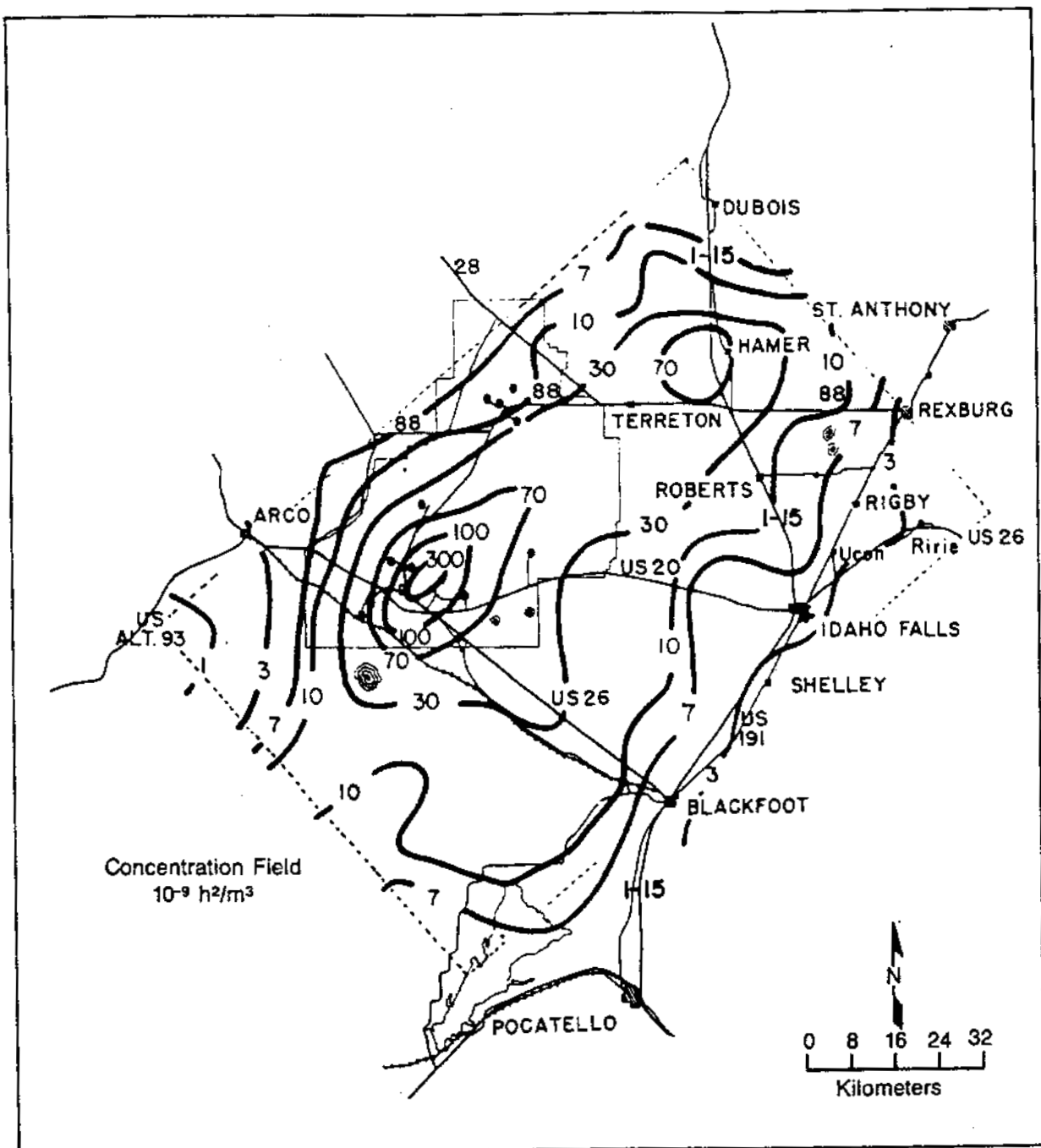
Figure B-16. 1977 average of mesoscale dispersion isopleths of air concentrations at ground level, normalized to unit release rate (DOE, 1978).
