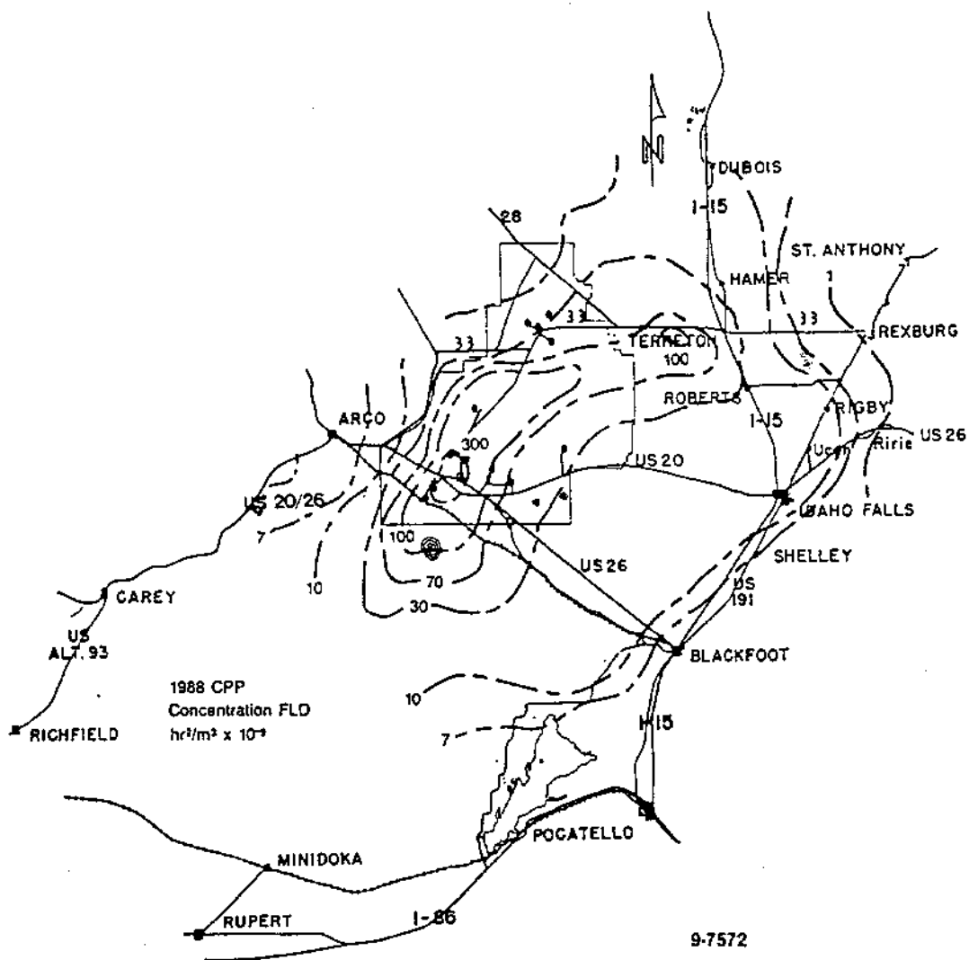
Figure B-6. 1988 average of mesoscale dispersion isopleths of air concentrations at ground level, normalized to unit release rate (Hoff et. al, 1989).
