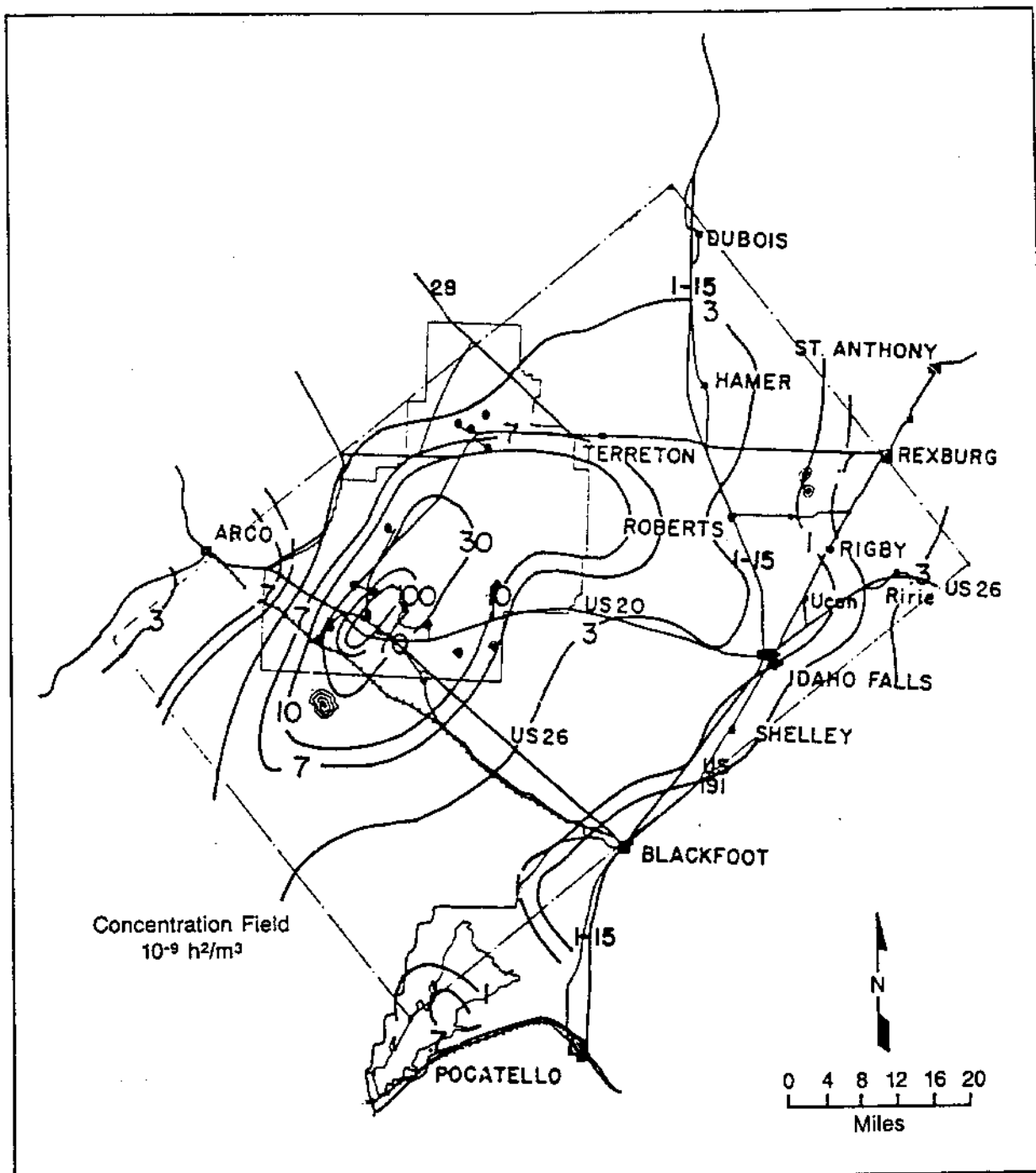
Figure B-19. 1974 average of mesoscale dispersion isopleths of air concentrations at ground level, normalized to unit release rate (ERDA, 1975).
