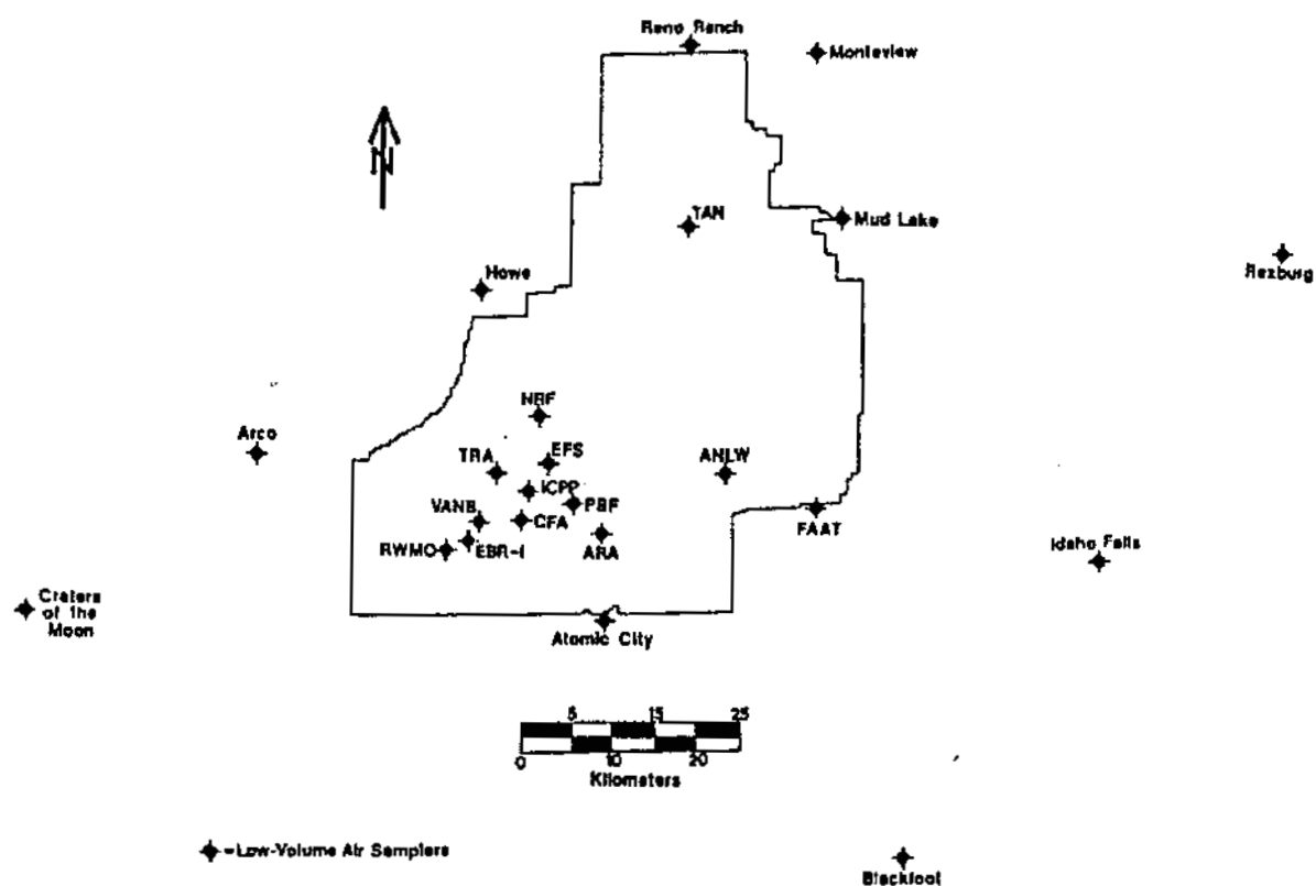
Figure E-1. INEL Site and vicinity air sampling network.
