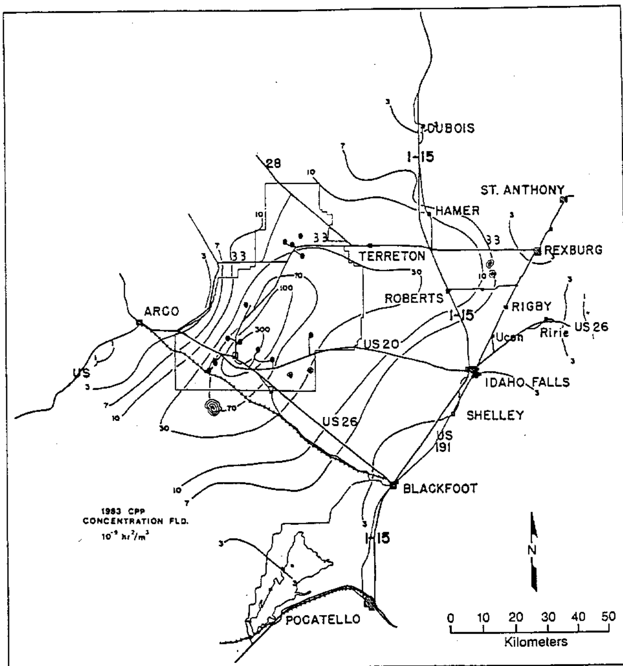
Figure B-11. 1983 average of mesoscale dispersion isopleths of air concentrations at ground level, normalized to unit release rate (Hoff et al., 1984).
