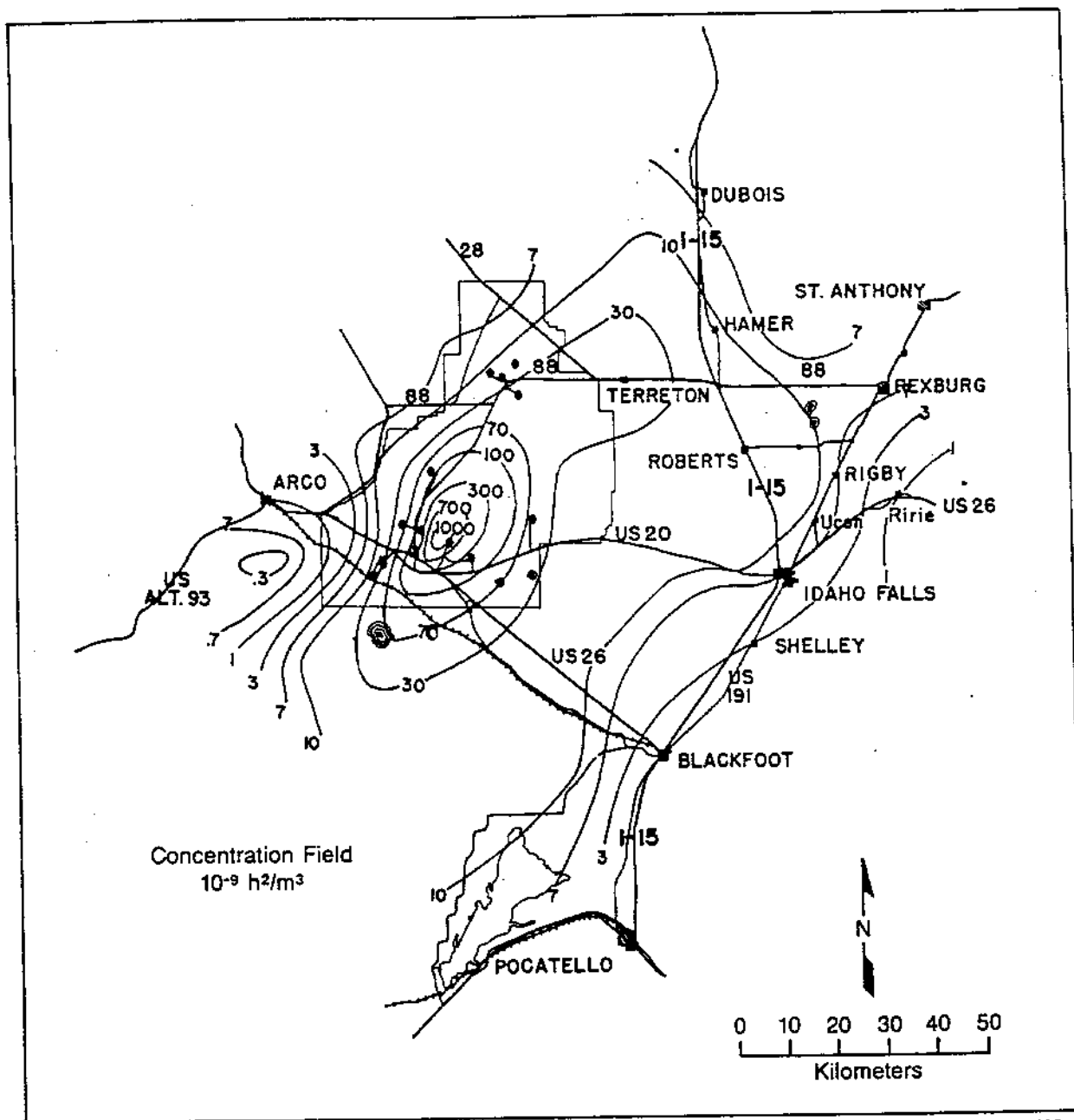
Figure B-15. 1979 average of mesoscale dispersion isopleths of air concentrations at ground level, normalized to unit release rate (DOE, 1980).
