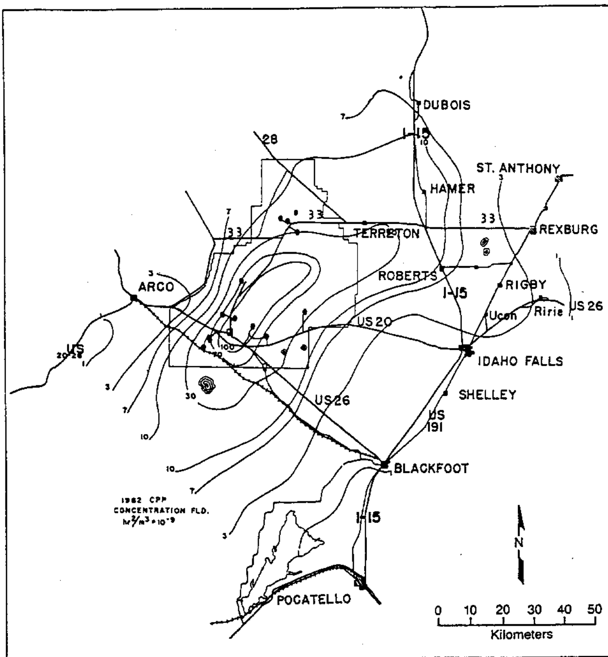
Figure B-12. 1982 average of mesoscale dispersion isopleths of air concentrations at ground level, normalized to unit release rate (DOE, 1983).
