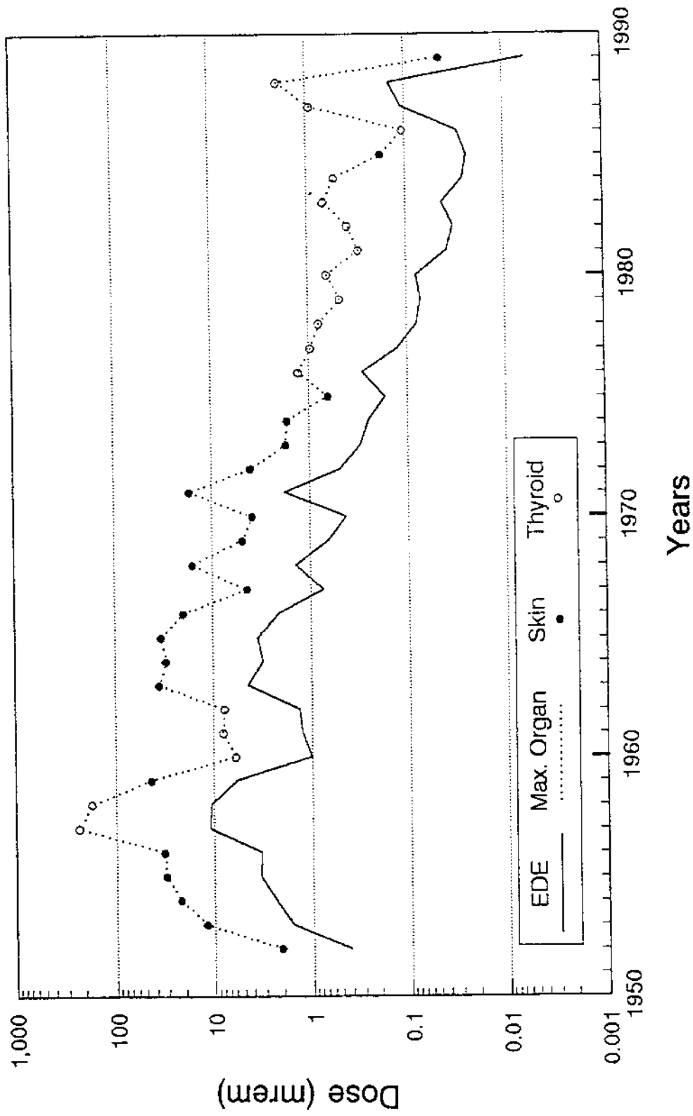
Figure C-1. Maximally exposed adult operational dose estimates.
