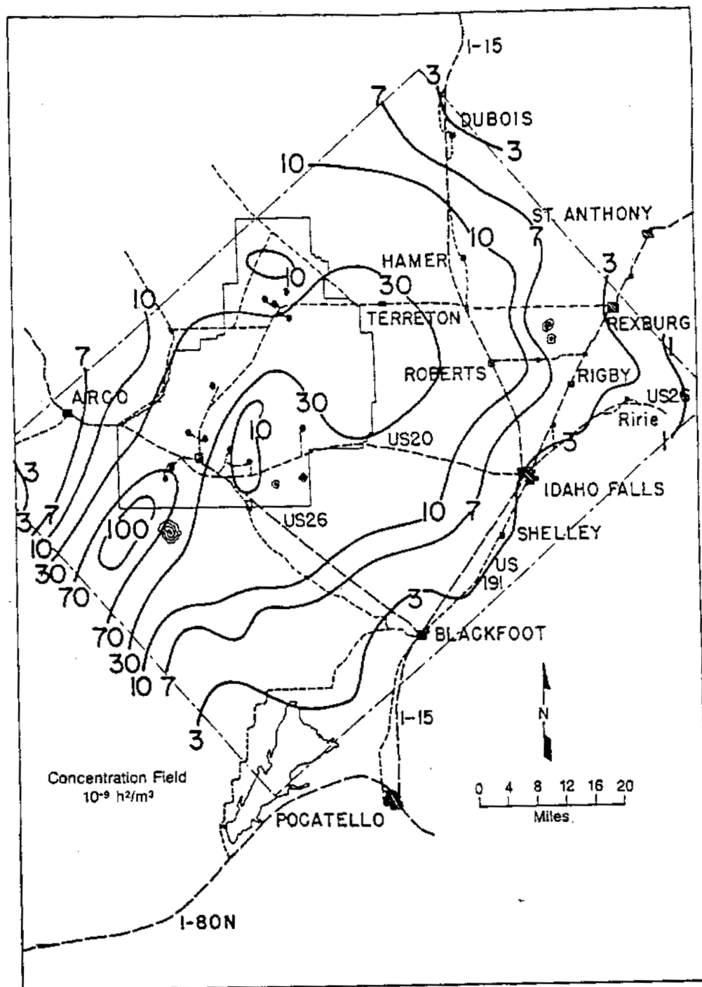
Figure B-20. 1973 average of mesoscale dispersion isopleths of air concentrations at ground level, normalized to unit release rate (AEC, 1974).
