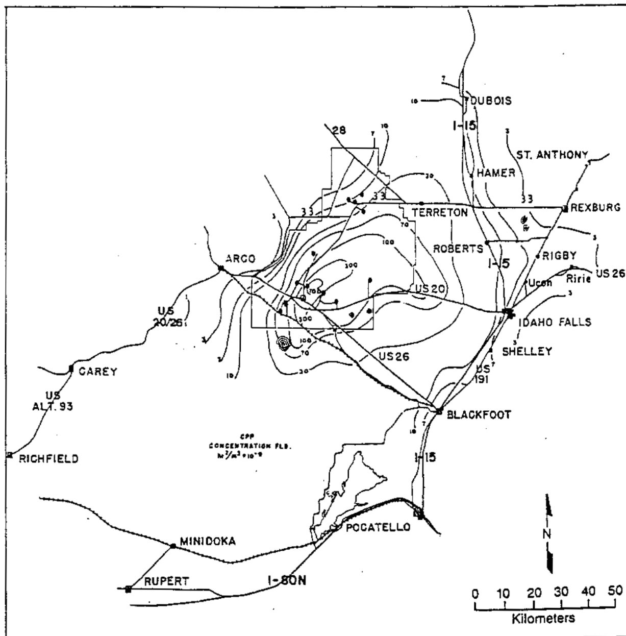
Figure B-9. 1985 average of mesoscale dispersion isopleths of air concentrations at ground level, normalized to unit release rate (Hoff et al., 1986).
