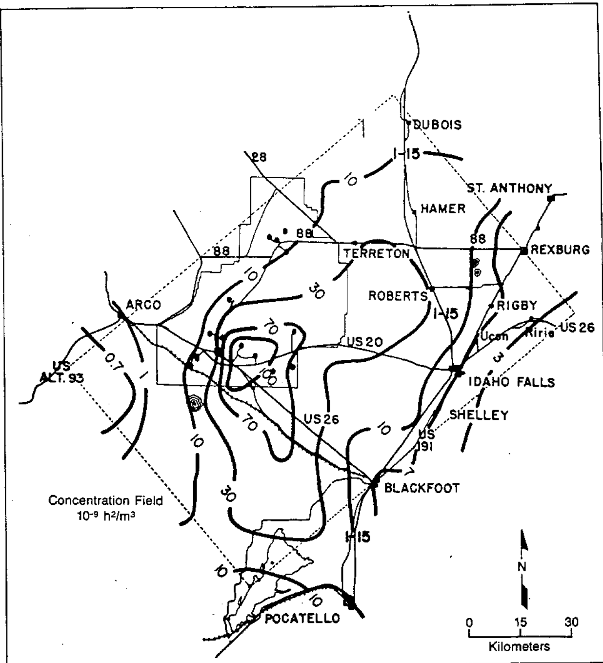
Figure B-17. 1976 average of mesoscale dispersion isopleths of air concentrations at ground level, normalized to unit release rate (ERDA, 1977).
