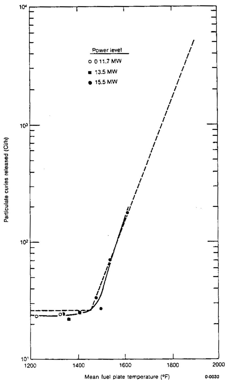
Figure A-3. IET #4 quantity of particulate activity.
