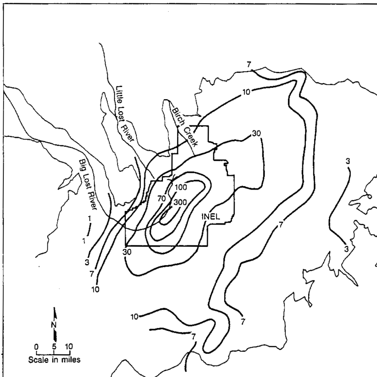
Figure B-4. Nine-year (1974-1983) average mesoscale dispersion isopleths of air concentration at ground level, normalized to unit release rate (Bowman, 1984).
