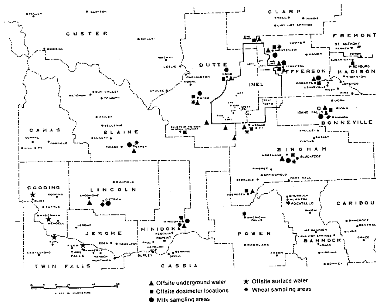
Figure E-4. Boundary and distant water, milk, and wheat sampling locations and environmental dosimeter locations.
