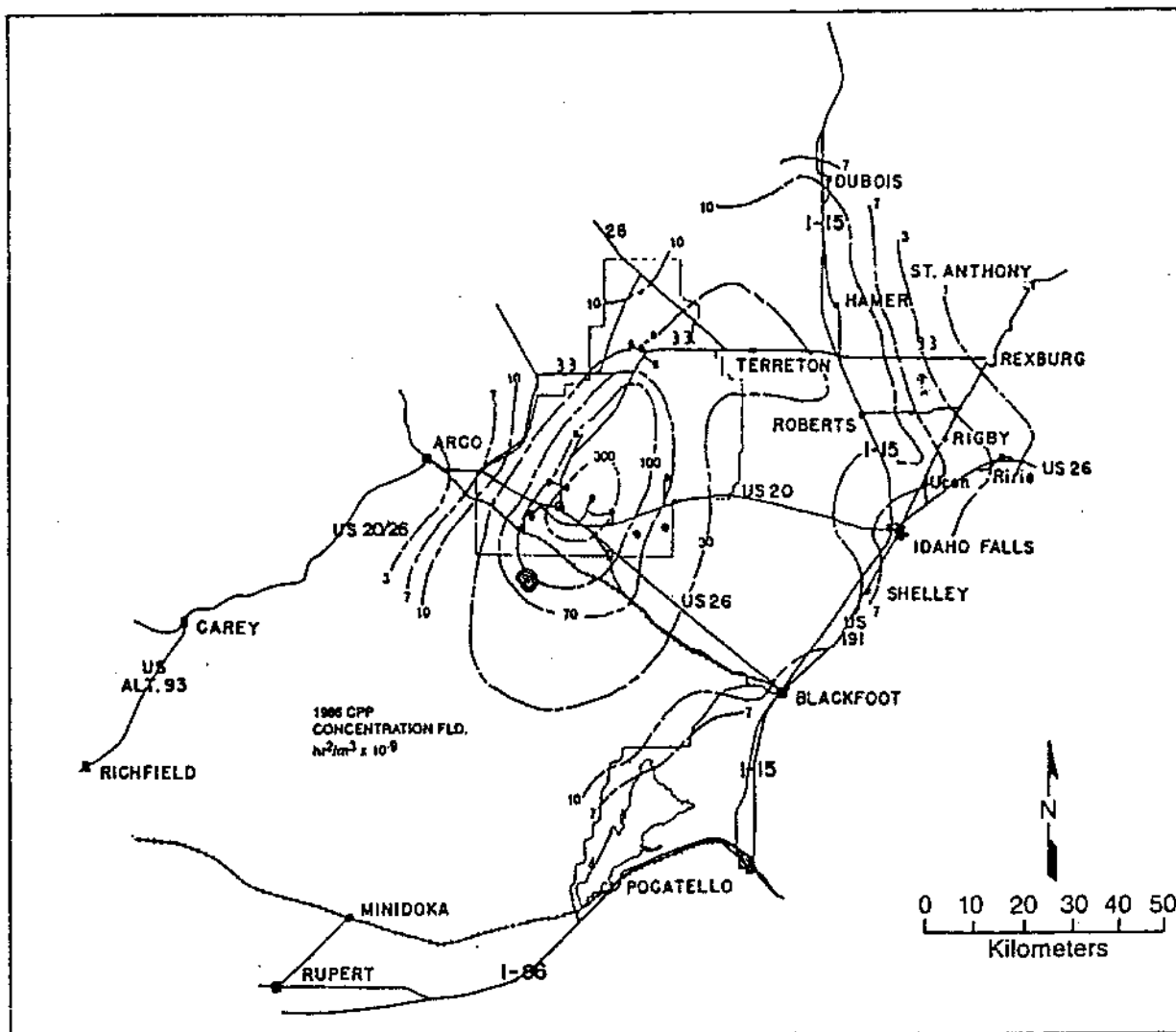
Figure B-8. 1986 average of mesoscale dispersion isopleths of air concentrations at ground level, normalized to unit release rate (Hoff et al., 1987).
