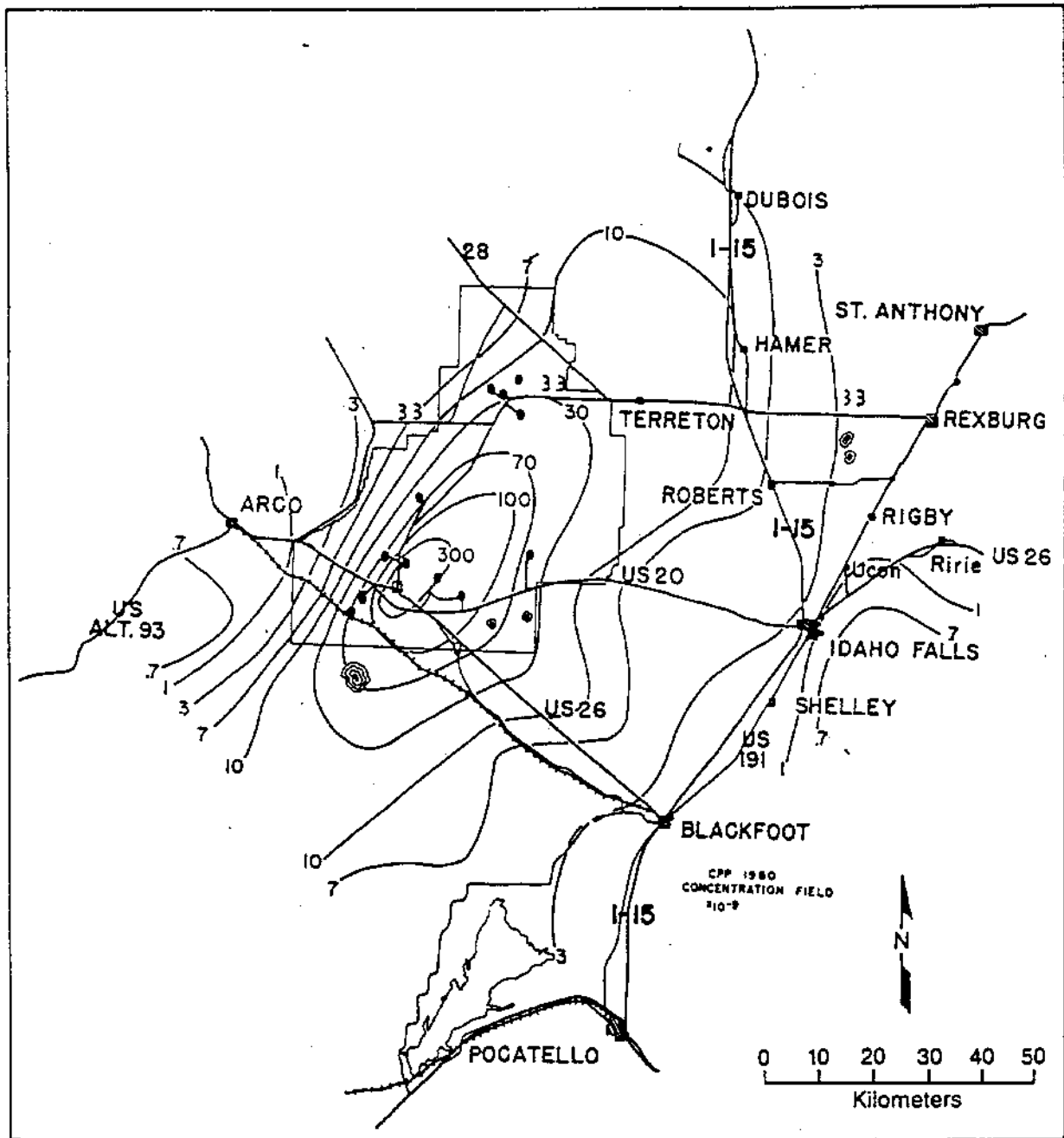
Figure B-14. 1980 average of mesoscale dispersion isopleths of air concentrations at ground level, normalized to unit release rate (DOE, 1981).
