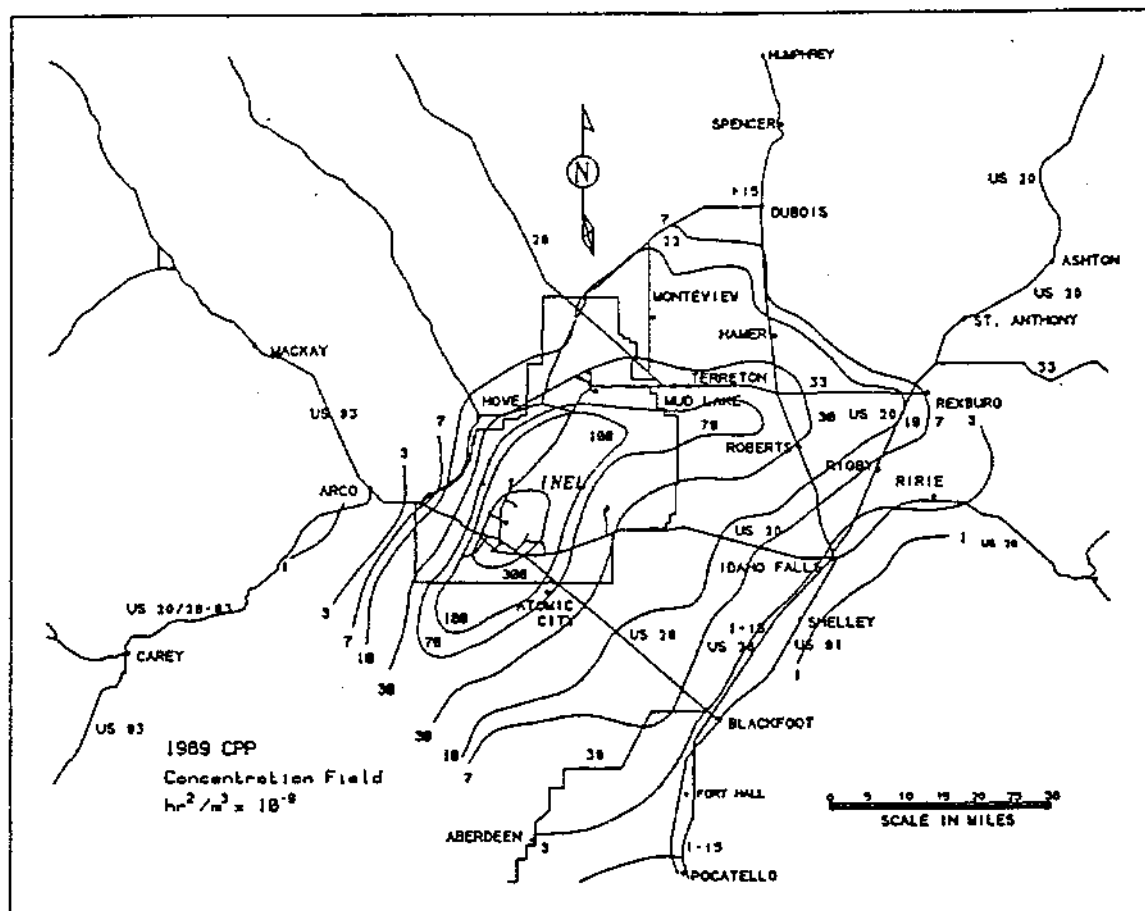
Figure B-5. 1989 average of mesoscale dispersion isopleths of air concentrations at ground level, normalized to unit release rate (Hoff et. al, 1990).
