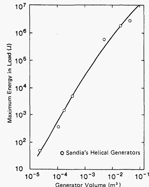
Maximum energy vs volume for seven established helical generator designs. Explosive-to-electric energy conversion efficiency improves as generator volume increases. Conversion efficiency is \sim 5\% for the largest generators.
