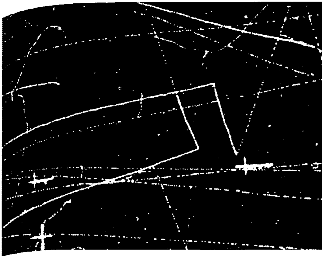
Mesons. Fragment of a hydrogen bubble chamber photograph showing, among other tracks, two pi-mesons coming from the left, each decaying into a mu-meson (short heavy track at about 90^\circ ), and these decaying into an electron (thin dotted track). Examination of about 1000 of these events has shown that more of the electrons are emitted in the backward direction than in the forward direction, with respect to the motion of the mu-meson.
