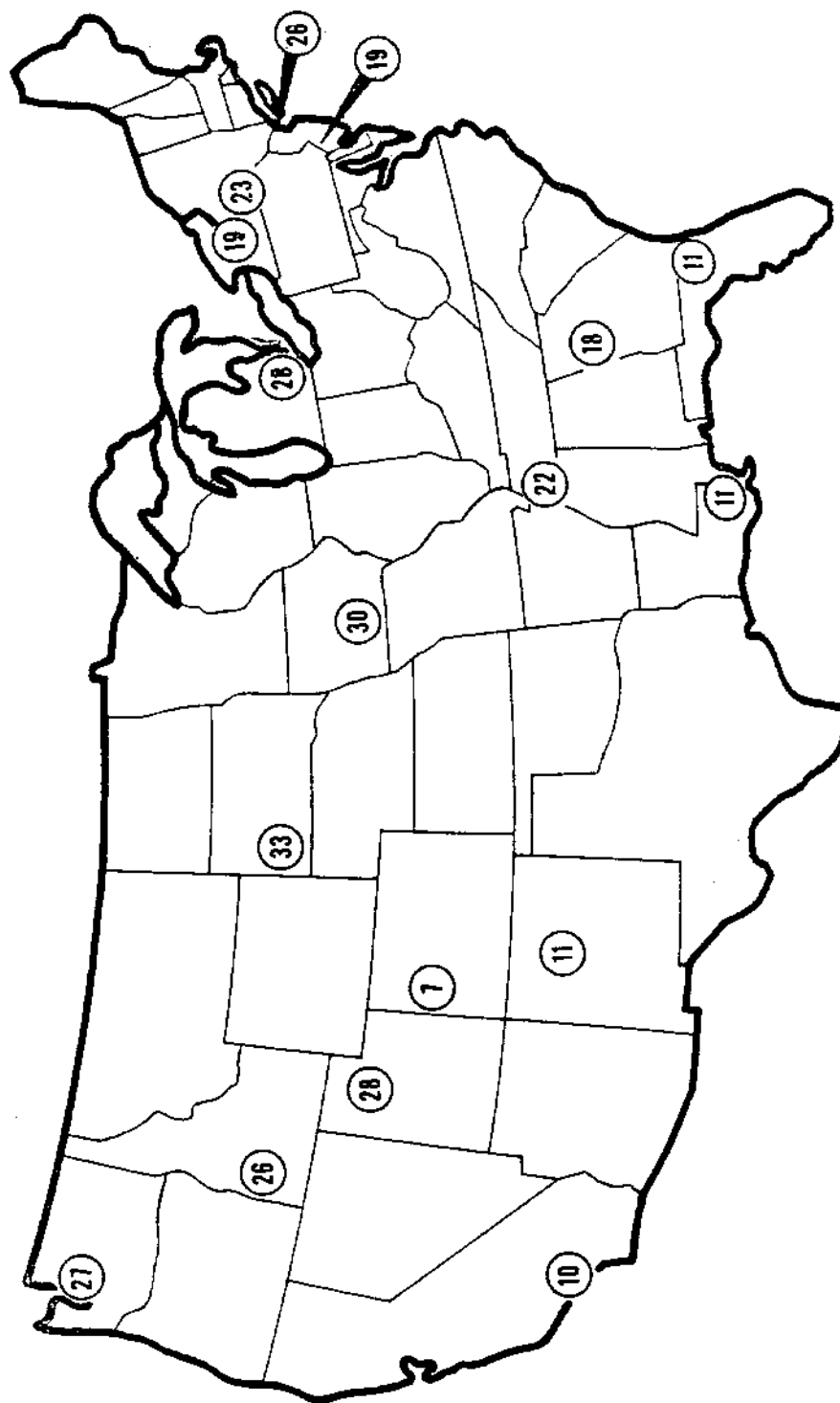
Fig. 5 S_{p90} IN U. S. SOIL (HASL - OCT. 8, 1956) (HCI EXTRACTION METHOD)
